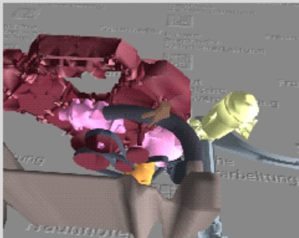
G. Zachmann, Color Plate II: Clash and clearance checks in the engine compartment by real-time collision detection. Parts colliding with the alternator are rendered in wireframe.
