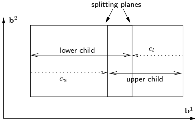
Figure 1: Child nodes are obtained from the parent node by splitting off one side of it. The drawing shows the case where a parent has a lower and an upper child that have coplanar splitting planes.
