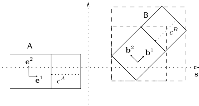
Figure 2: Only one value per axis s needs to be recomputed for the overlap test.
