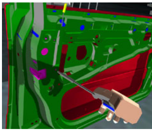
Fig. 12. Tools snap onto screws and are constrained. Also, they are placed automatically at an ergonomic position within the hand by the system.
