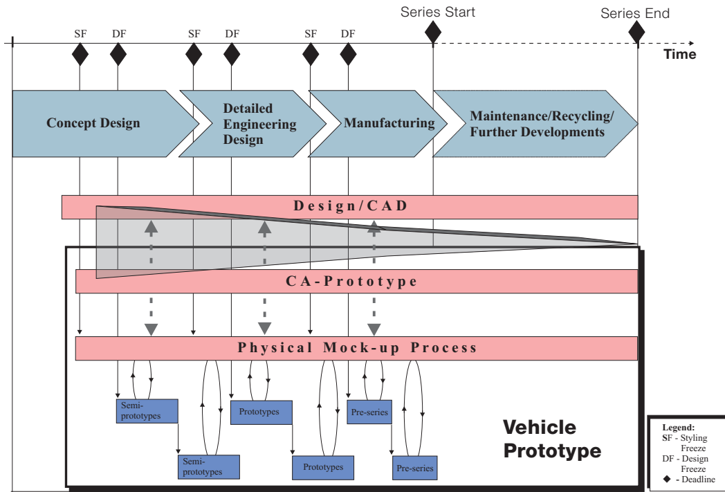
Fig. 1. Process chain for the vehicle prototype activities.
