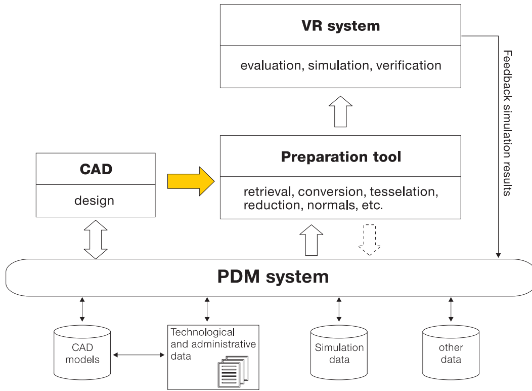
Fig. 3. Data flow between CAD and VR system.
