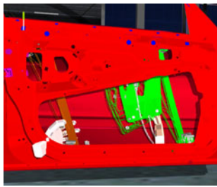
Fig. 13. The window regulator has to be installed with two hands; the “ghost” paradigm signals collisions.
