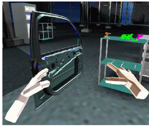
Fig. 8. The door scenario. Two hands and several tools are necessary to perform the assembly.
